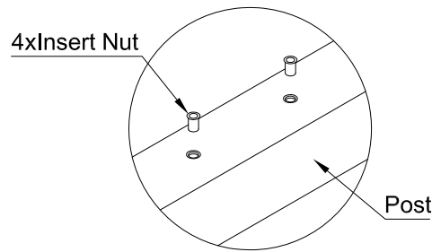
DETAIL B
